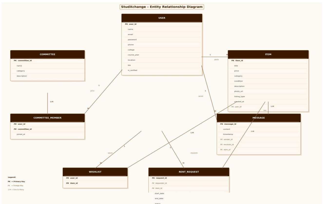
Fig 11 – Entity Relationship Diagram (StudXchange Database)
