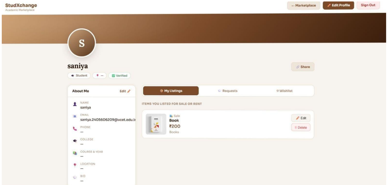
Fig 8 – My Profile Page
